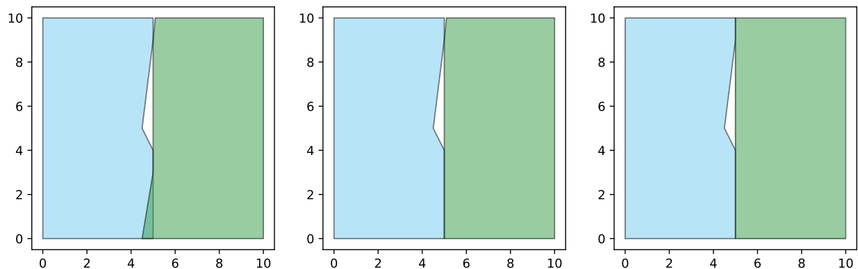
Fig. 14: Polygon dataset before cleaning (left), after cleaning with default snapping distance (center), and a more aggressive --snapping-distance 0.2 (right). Note the movement in the upper-left corner of the polygon on the right.
