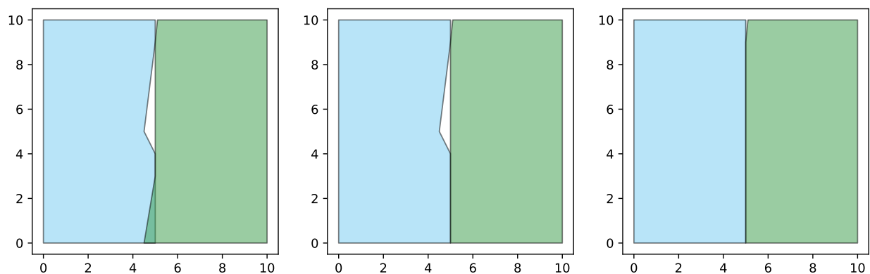
Fig. 12: Polygon dataset before cleaning (left), after cleaning with default parameters (center), and after cleaning with --maximum-gap-width 1 (right).
