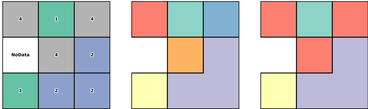
Fig. 2: Polygonization of a 3x3 raster input. The middle figure shows the default behavior, where separate polygons are created for pixel regions that are connected only to a diagonal neighbor. In the figure on the right, --connect-diagonal-pixels has been specified, and a single polygon has been created for pixels with value 4.
