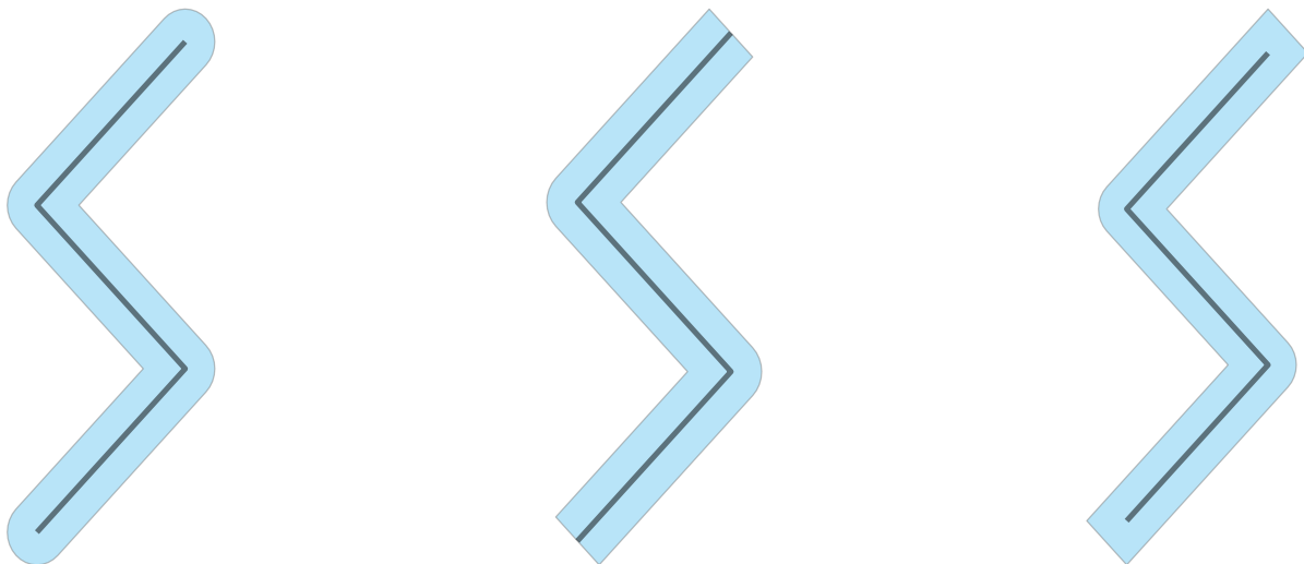
Fig. 5: Buffered lines with endcap-style=round, endcap-style=flat and endcap-style=square
