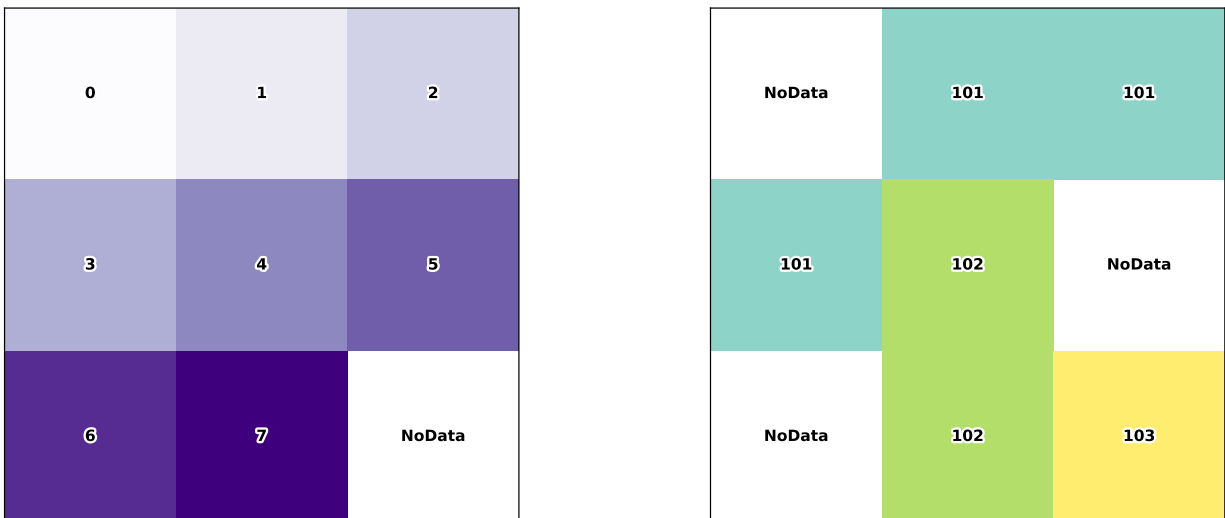
Fig. 3: Raster dataset before (left) and after (right) reclassification with gdal raster reclassify --mapping "[1,3]= 101; [4, 5)= 102; 7=102; NO_DATA=103; DEFAULT=NO_DATA" .
