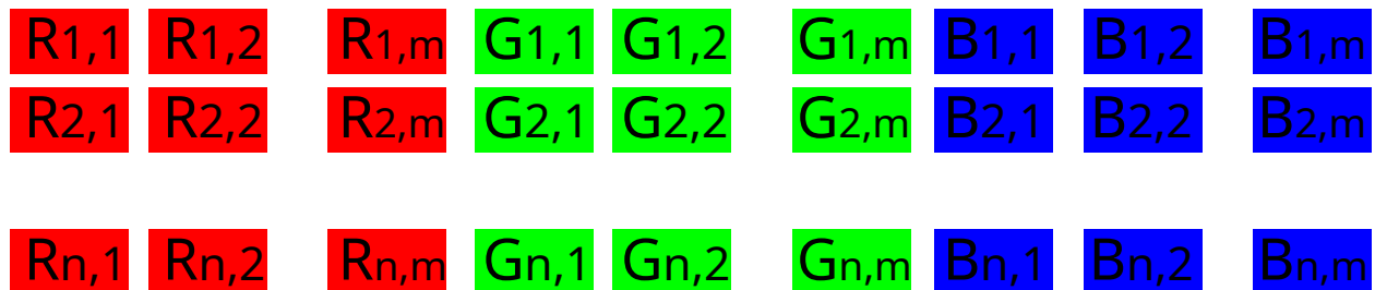
Fig. 3: Band Interleaved by Line (BIL) mode
