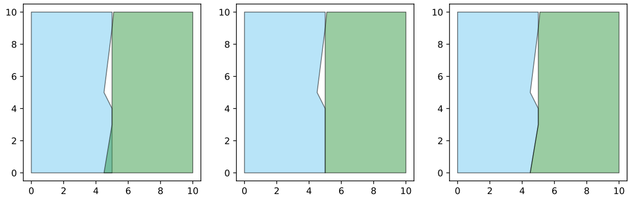
Fig. 13: Polygon dataset before cleaning (left), after cleaning with "longest-border" merge strategy (center) and --merge-strategy max-area (right).
