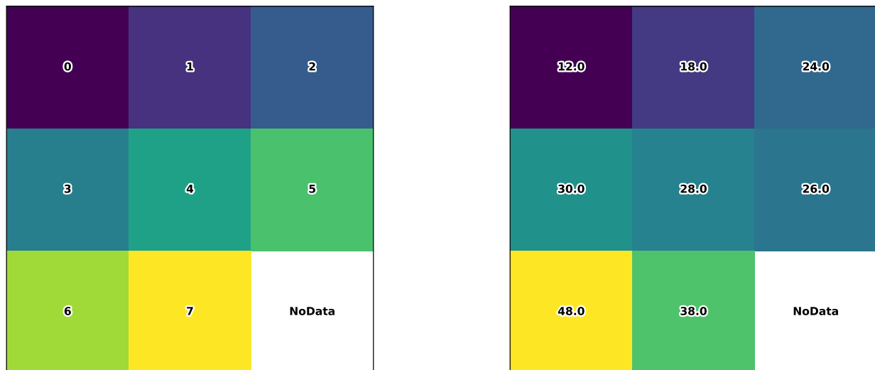
Fig. 1: Raster dataset before (left) and after (right) summation with a 3x3 equal-weight kernel. NoData values are considered zero for the purpose of the summation. Edge cells are replicated where the kernel window extends beyond the edge of the dataset.
