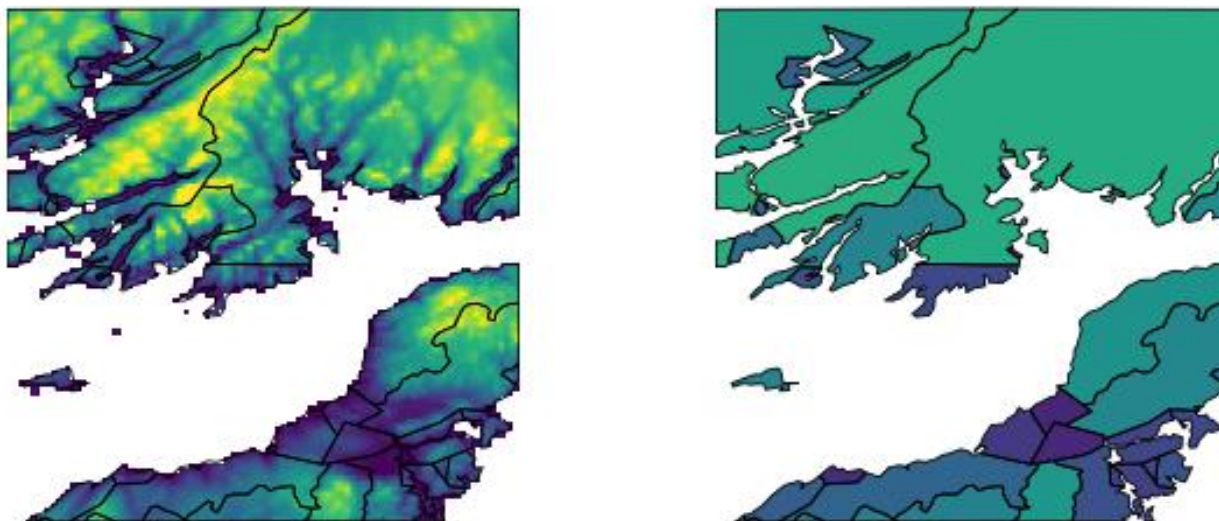
Fig. 4: Mean elevation calculated for each polygon from an elevation raster.
